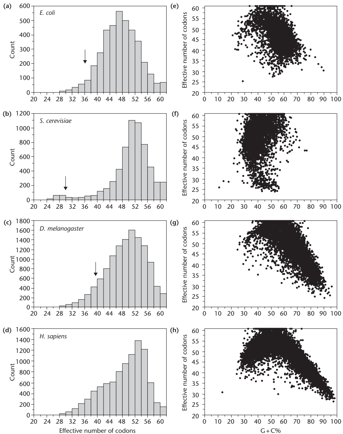
0102.F001 Figure 1 Codon usage bias in different organisms. (a, e) Escherichia coli , (b, f) Saccharomyces cerevisiae , (c, g) Drosophila melanogaster and (d, h) Homo sapiens . Codon usage bias is measured by the 'effective number of codons' ( N_c ). 'G+C%' is the G+C content at third-codon positions. The sources for the sequence data are given in Table 1 . The average N_c for each organism is 47.3 for E. coli , 50.6 for S. cerevisiae , 49.2 for D. melanogaster and 48.7 for H. sapiens . Arrowheads indicate the average N_c for ribosomal protein genes (including predicted genes) with more than 100 codons. The number of ribosomal protein genes included (and the average N_c ) for each organism is 39 (36.3) for E. coli , 102 (29.9) for S. cerevisiae and 94 (39.3) for D. melanogaster .
